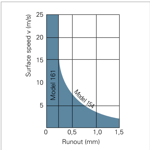
Diagram 2: Runout absorption
